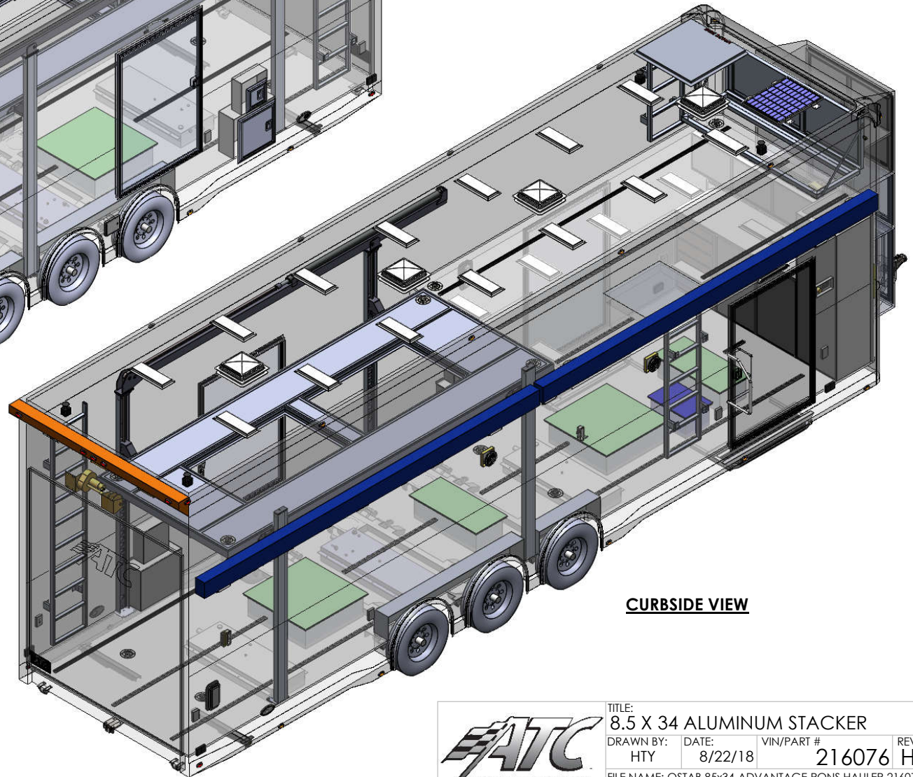
ROADSIDE VIEW
